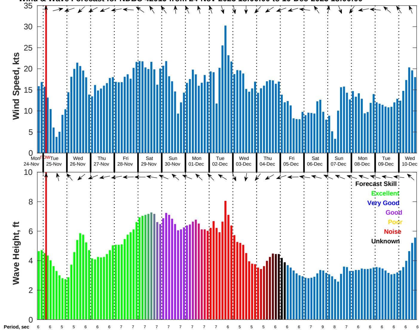
Wind & Wave Forecast for NDBC 42019 from 24-Nov-2025 18:00:00 to 10-Dec-2025 18:00:00
