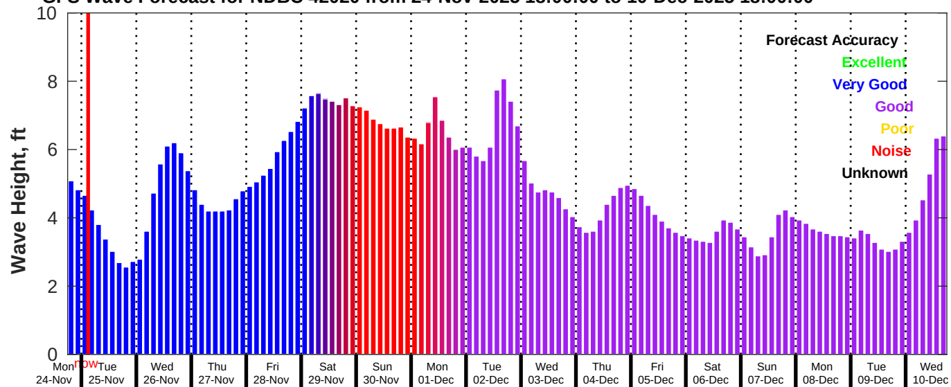
GFS Wave Forecast for NDBC 42020 from 24-Nov-2025 18:00:00 to 10-Dec-2025 18:00:00
