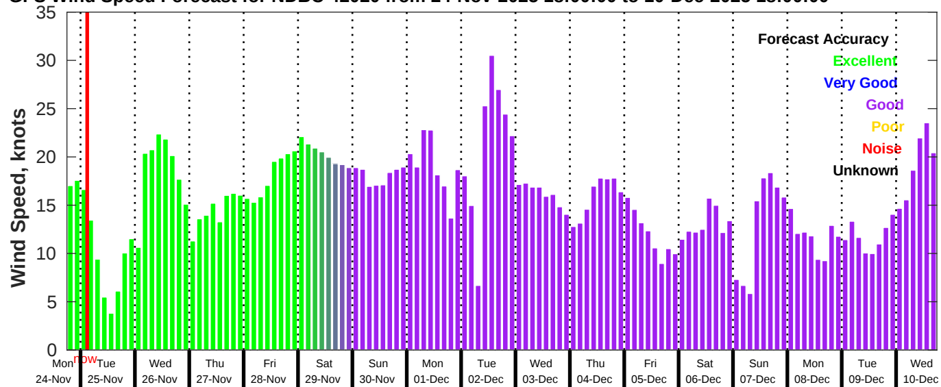
GFS Wind Speed Forecast for NDBC 42020 from 24-Nov-2025 18:00:00 to 10-Dec-2025 18:00:00
