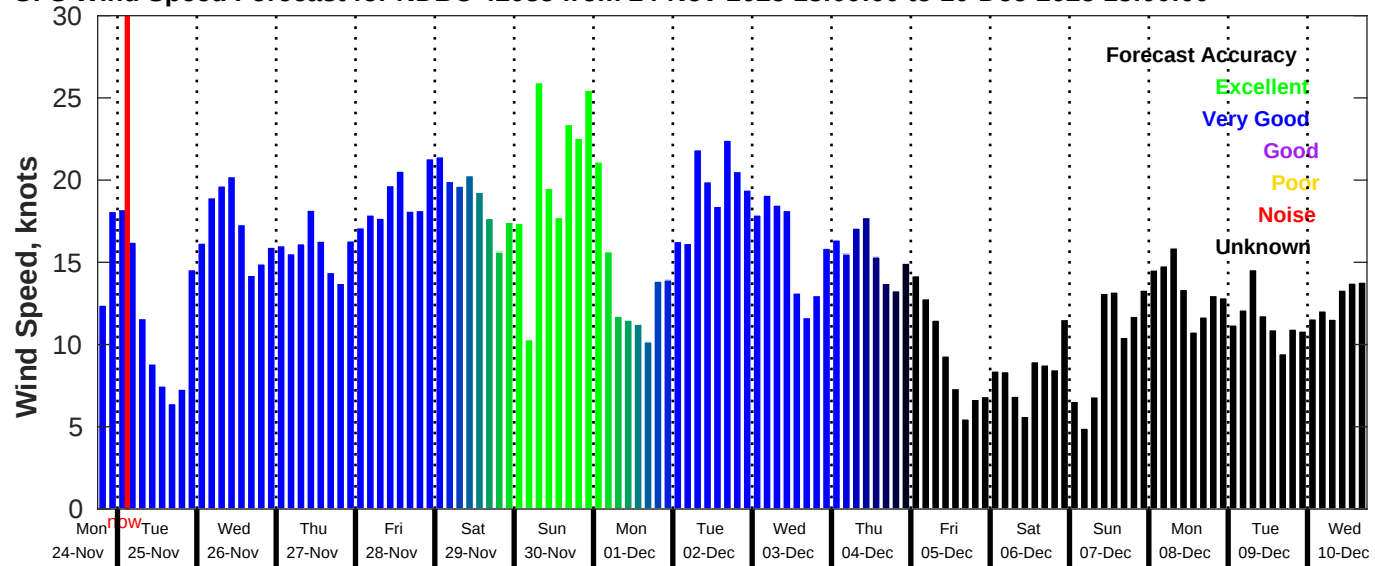
GFS Wind Speed Forecast for NDBC 42035 from 24-Nov-2025 18:00:00 to 10-Dec-2025 18:00:00
