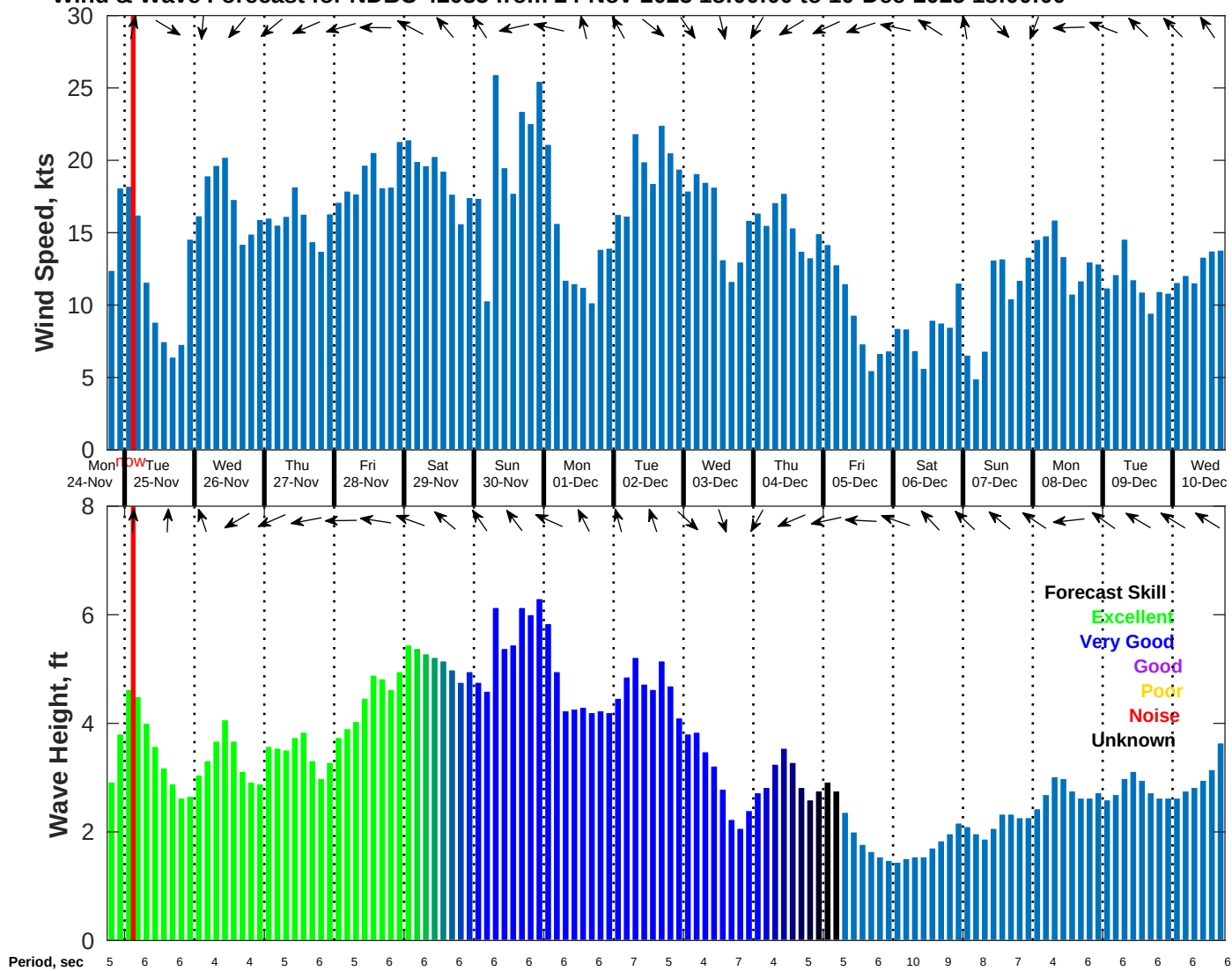
Wind & Wave Forecast for NDBC 42035 from 24-Nov-2025 18:00:00 to 10-Dec-2025 18:00:00
