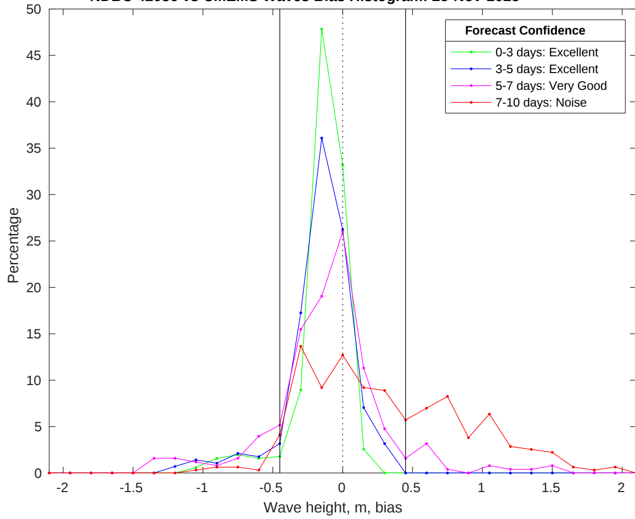
NDBC 42036 vs CMEMS Waves Bias Histogram: 25-Nov-2025
