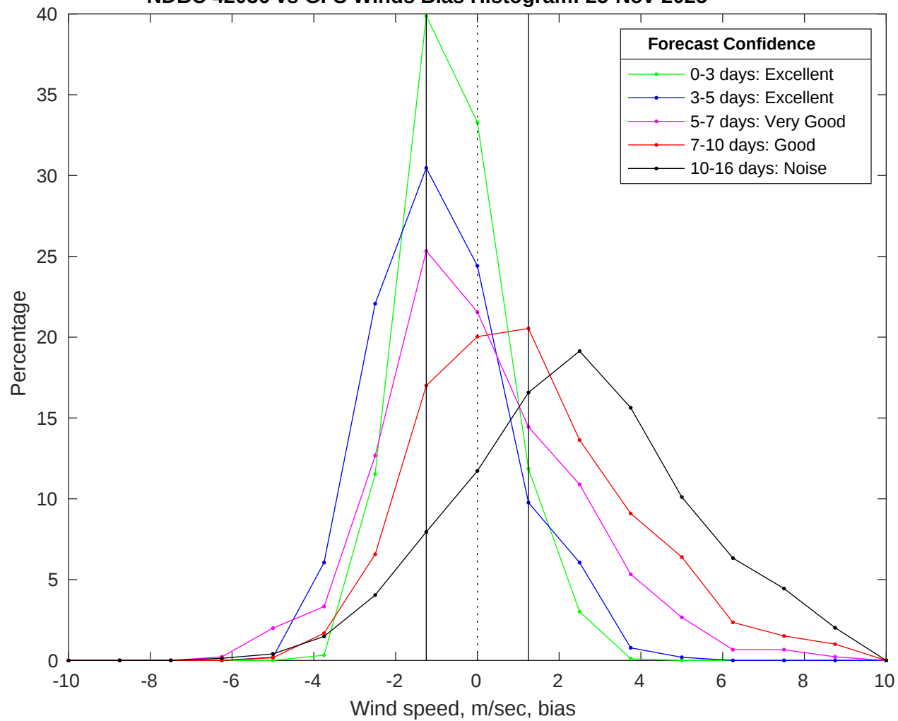
NDBC 42036 vs GFS Winds Bias Histogram: 25-Nov-2025
