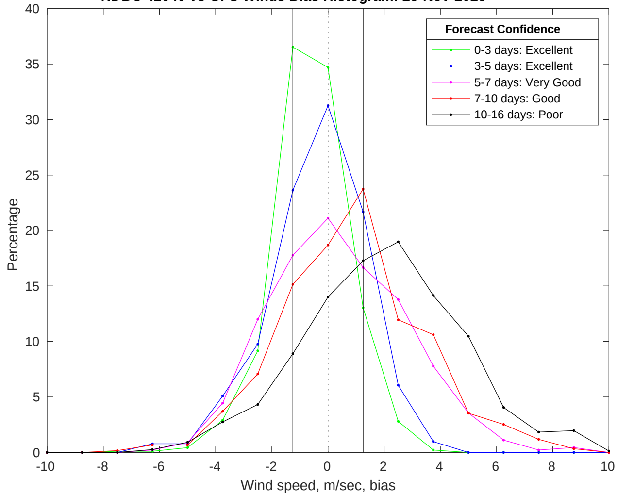
NDBC 42040 vs GFS Winds Bias Histogram: 25-Nov-2025
