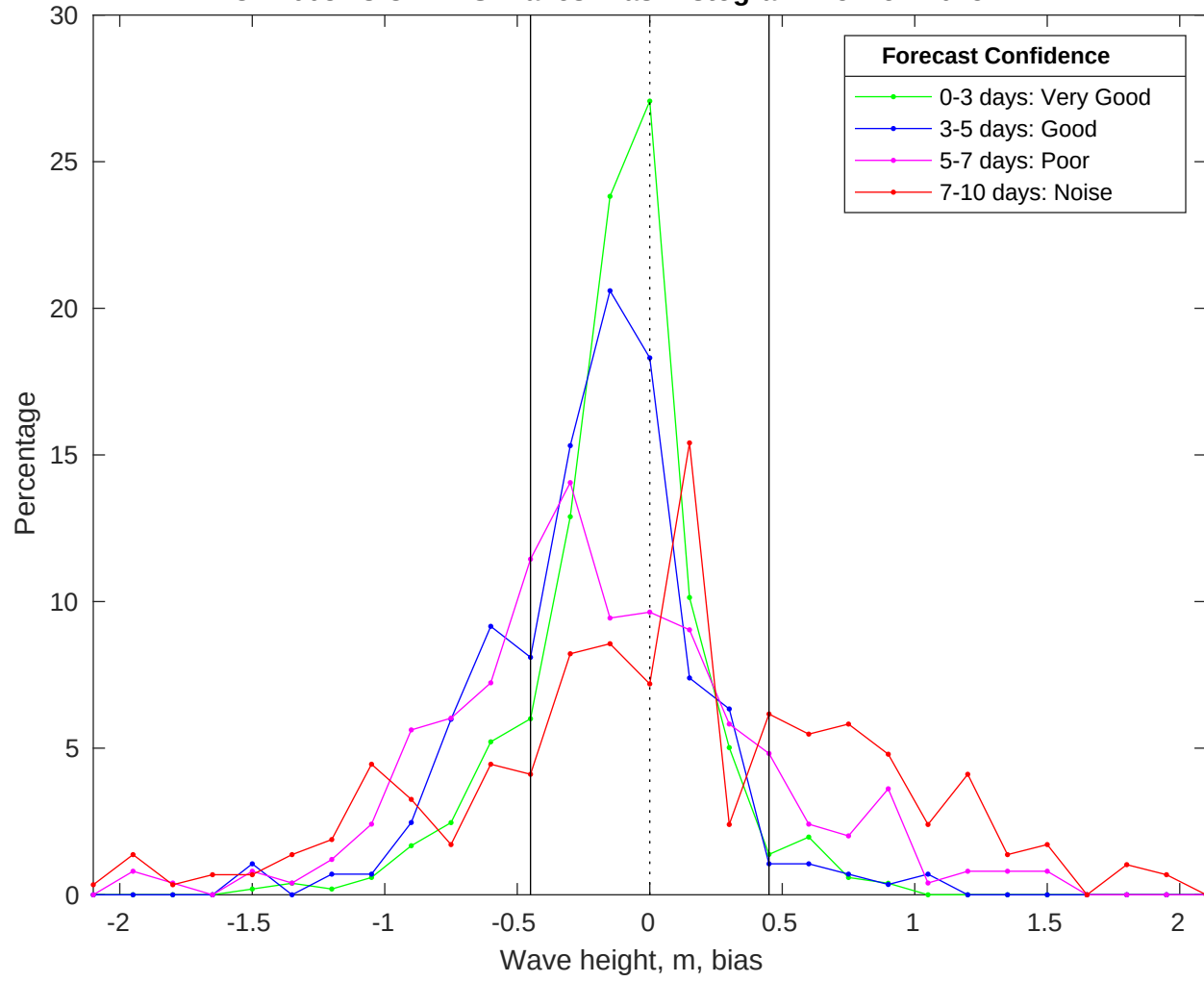
NDBC 44008 vs CMEMS Waves Bias Histogram: 25-Nov-2025
