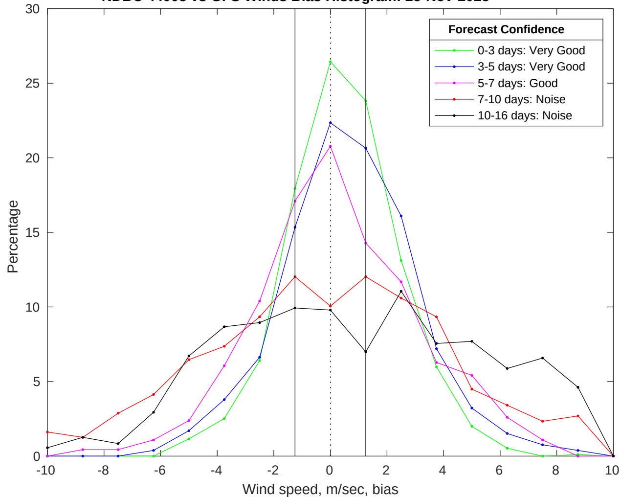
NDBC 44008 vs GFS Winds Bias Histogram: 25-Nov-2025
