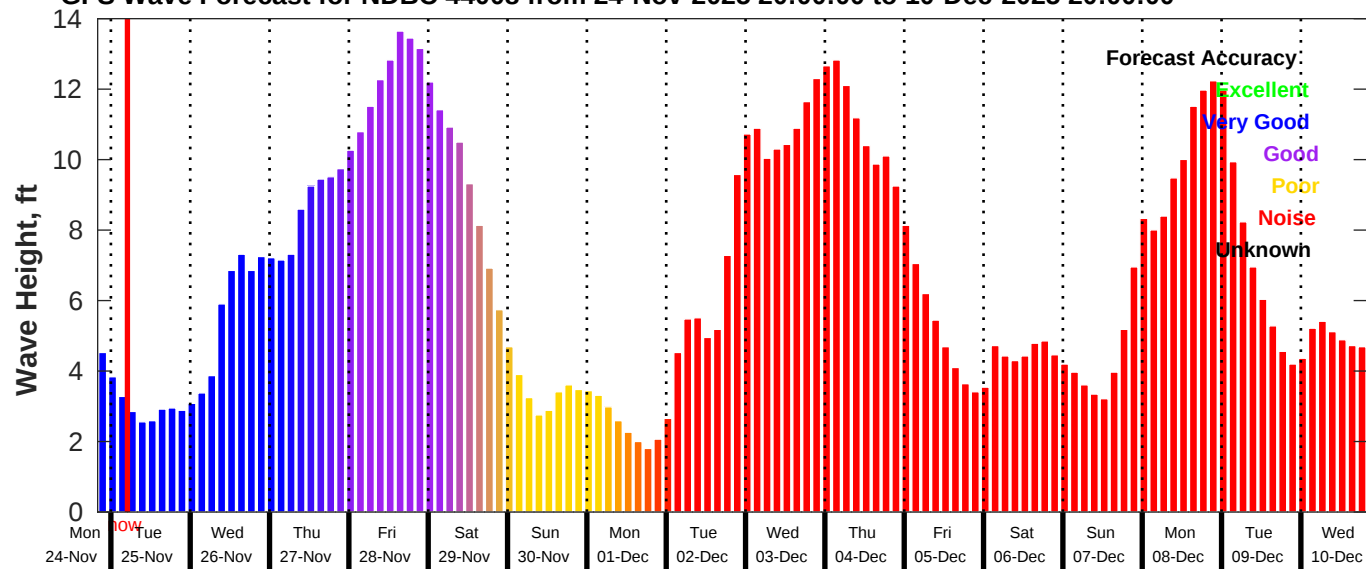
GFS Wave Forecast for NDBC 44008 from 24-Nov-2025 20:00:00 to 10-Dec-2025 20:00:00
