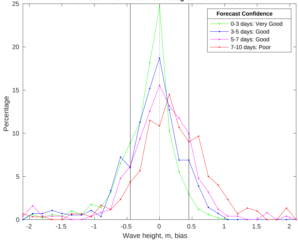
NDBC 46011 vs CMEMS Waves Bias Histogram: 25-Nov-2025
