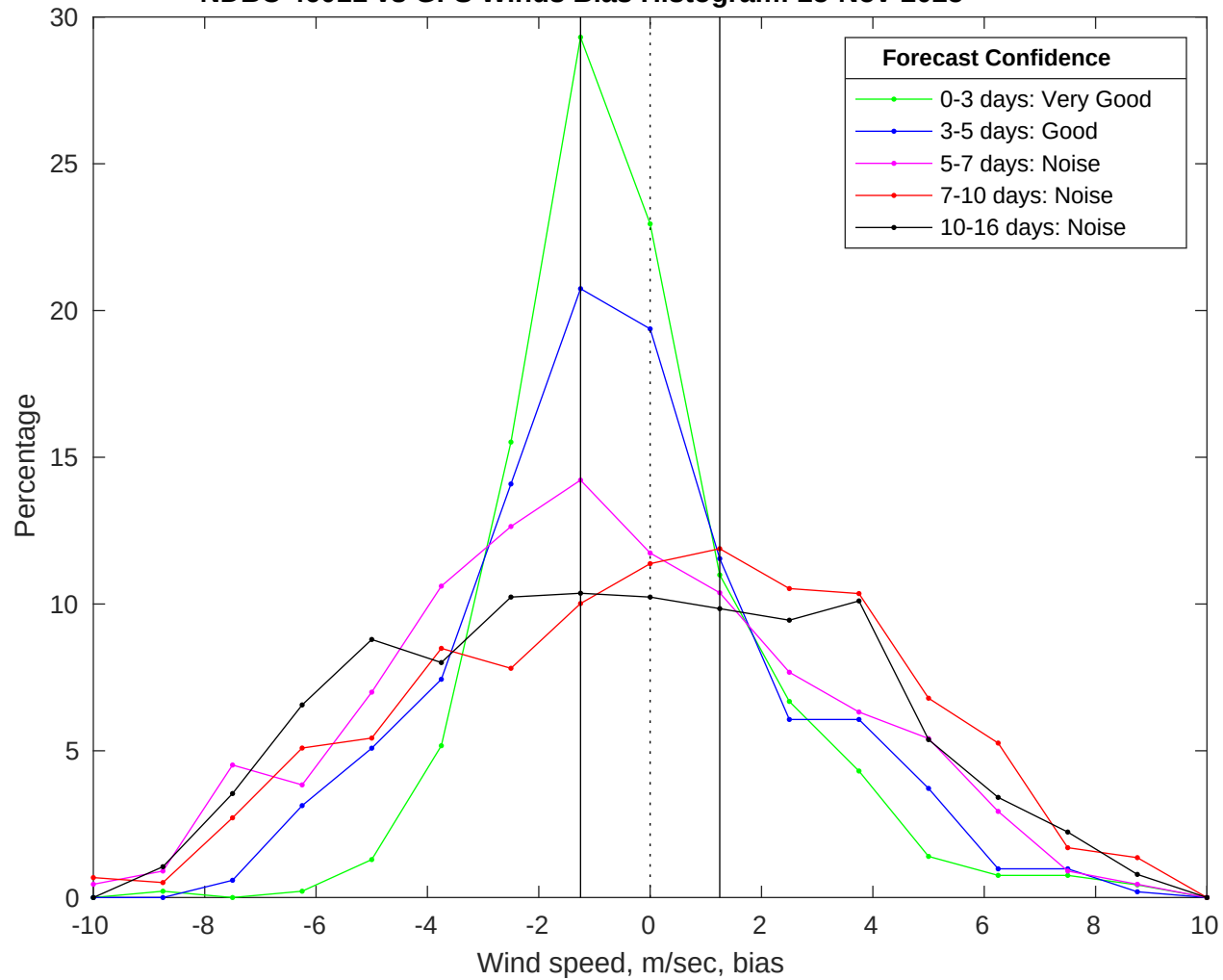
NDBC 46011 vs GFS Winds Bias Histogram: 25-Nov-2025
