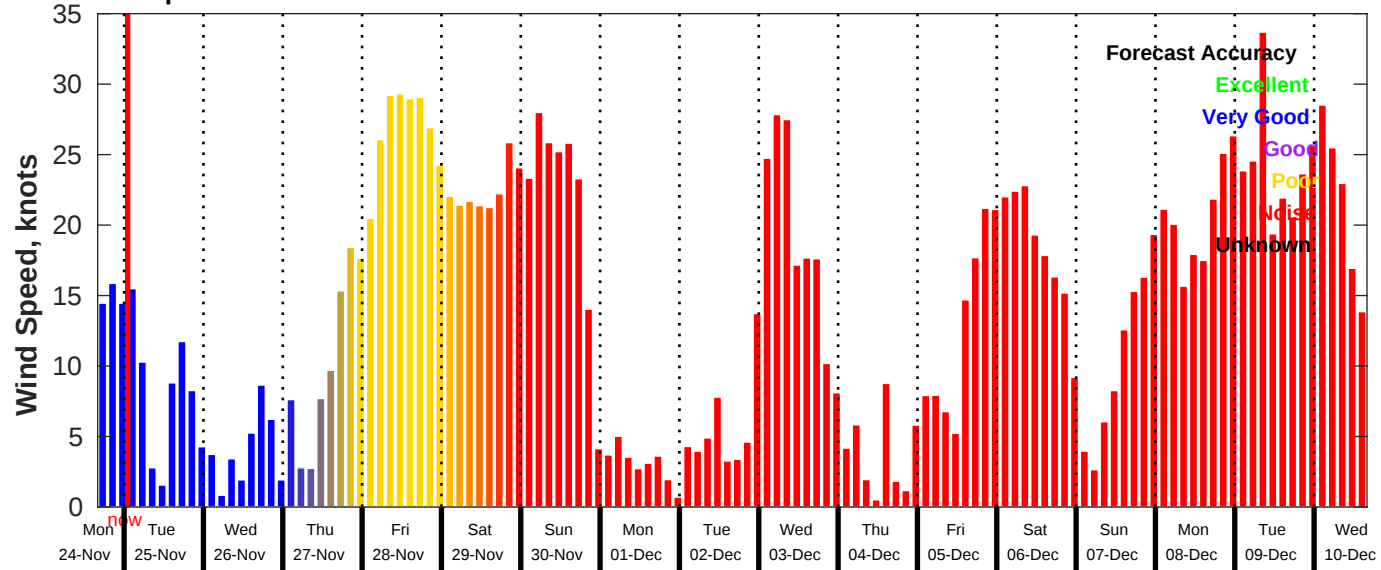
GFS Wind Speed Forecast for NDBC 46028 from 24-Nov-2025 16:00:00 to 10-Dec-2025 16:00:00
