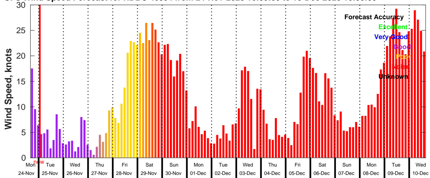
GFS Wind Speed Forecast for NDBC 46054 from 24-Nov-2025 16:00:00 to 10-Dec-2025 16:00:00
