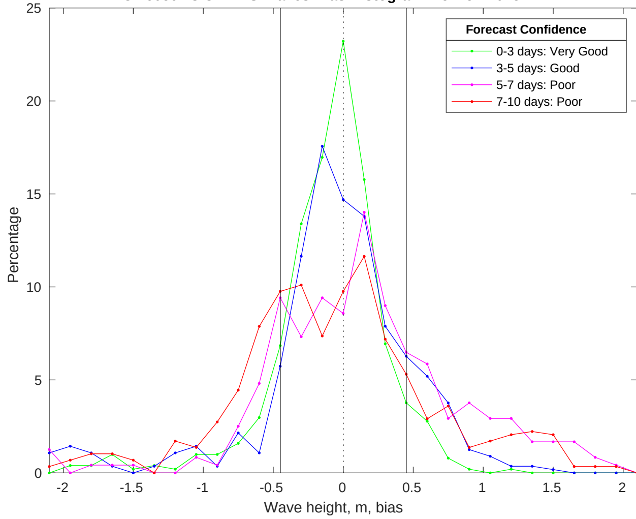
NDBC 46059 vs CMEMS Waves Bias Histogram: 25-Nov-2025
