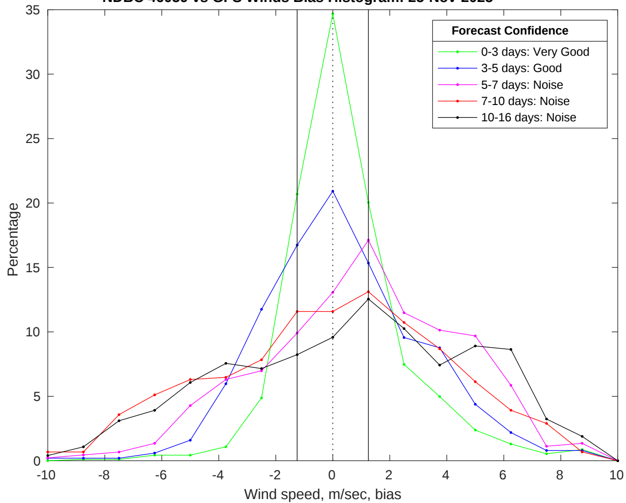
NDBC 46059 vs GFS Winds Bias Histogram: 25-Nov-2025
