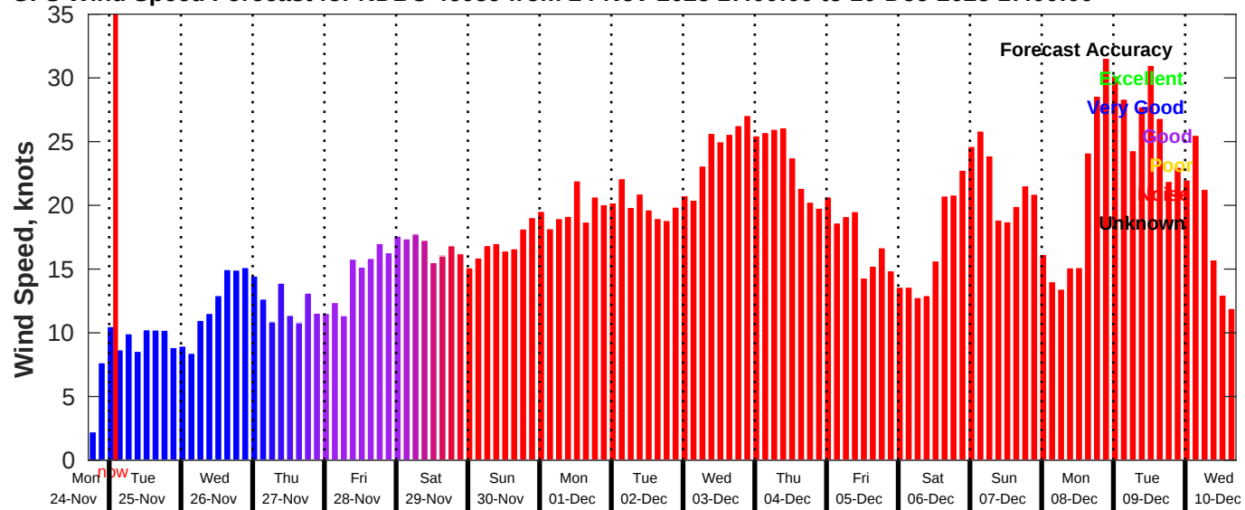
GFS Wind Speed Forecast for NDBC 46059 from 24-Nov-2025 17:00:00 to 10-Dec-2025 17:00:00
