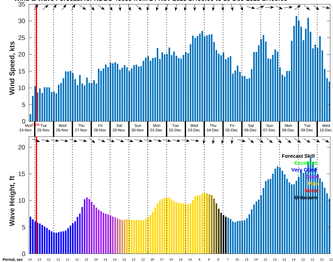
Wind & Wave Forecast for NDBC 46059 from 24-Nov-2025 17:00:00 to 10-Dec-2025 17:00:00
