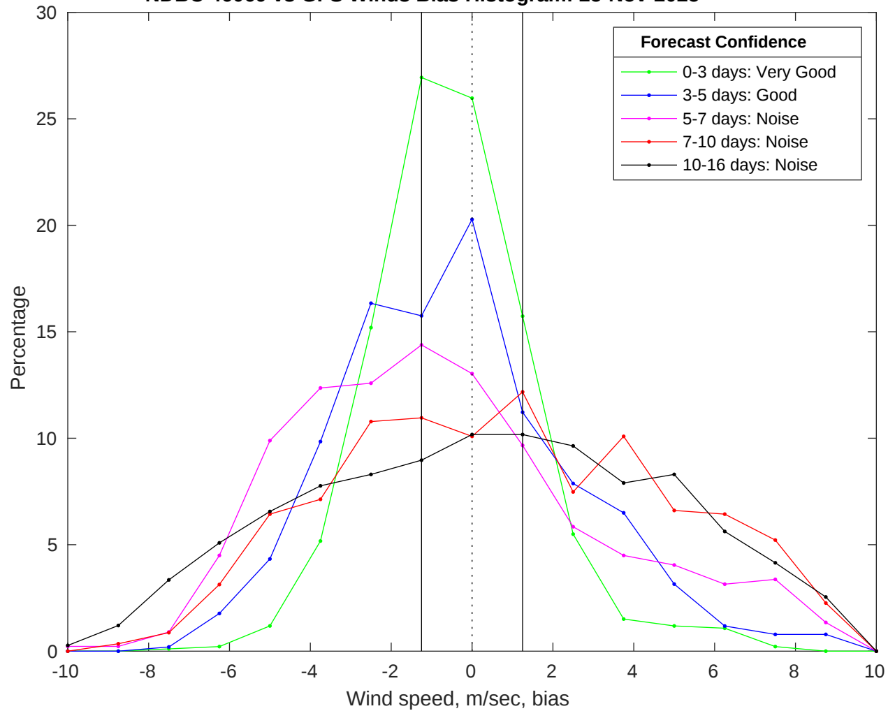
NDBC 46069 vs GFS Winds Bias Histogram: 25-Nov-2025
