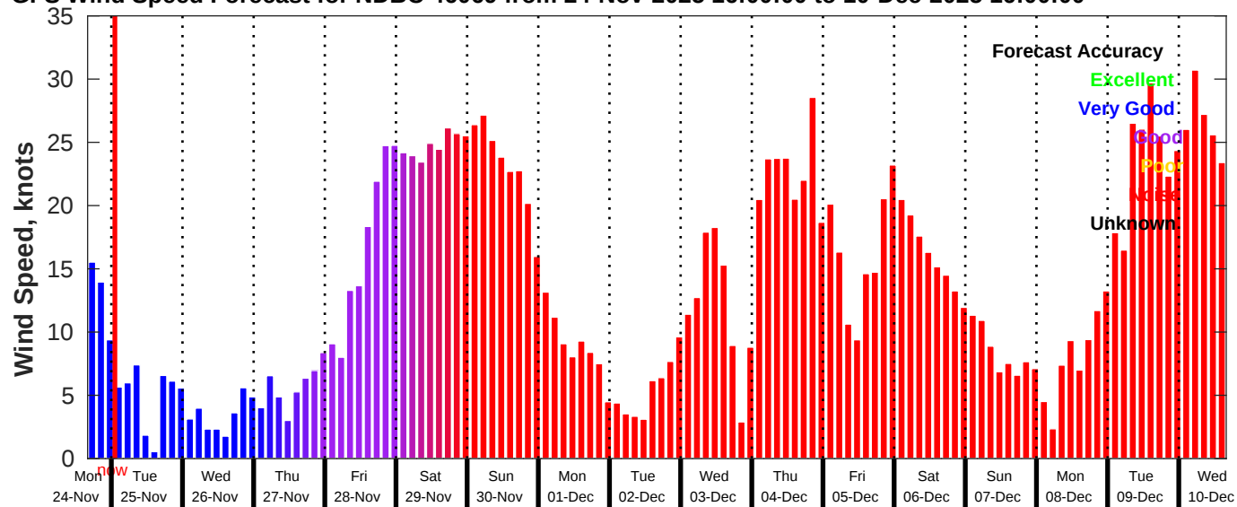
GFS Wind Speed Forecast for NDBC 46069 from 24-Nov-2025 16:00:00 to 10-Dec-2025 16:00:00
