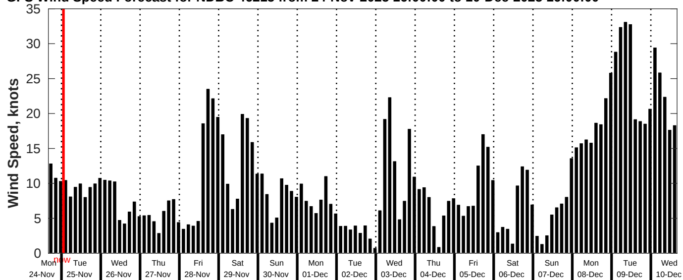
GFS Wind Speed Forecast for NDBC 46215 from 24-Nov-2025 16:00:00 to 10-Dec-2025 16:00:00
