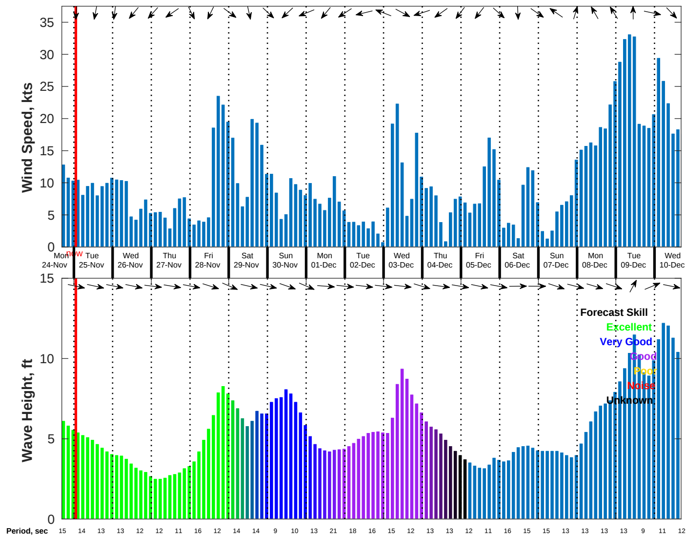
Wind & Wave Forecast for NDBC 46215 from 24-Nov-2025 16:00:00 to 10-Dec-2025 16:00:00
