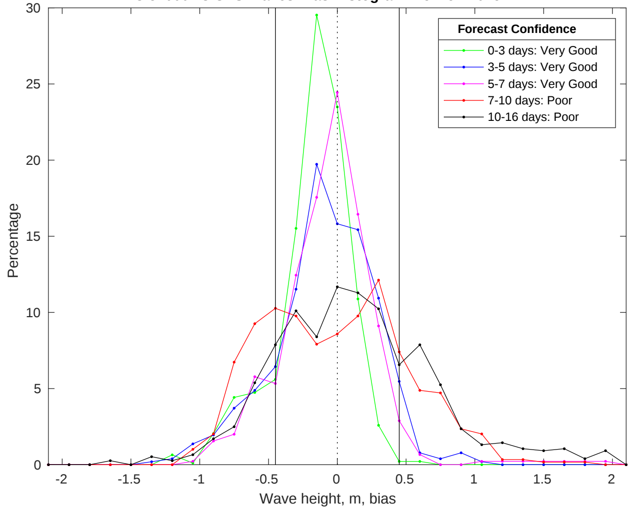
NDBC 51000 vs GFS Waves Bias Histogram: 25-Nov-2025
