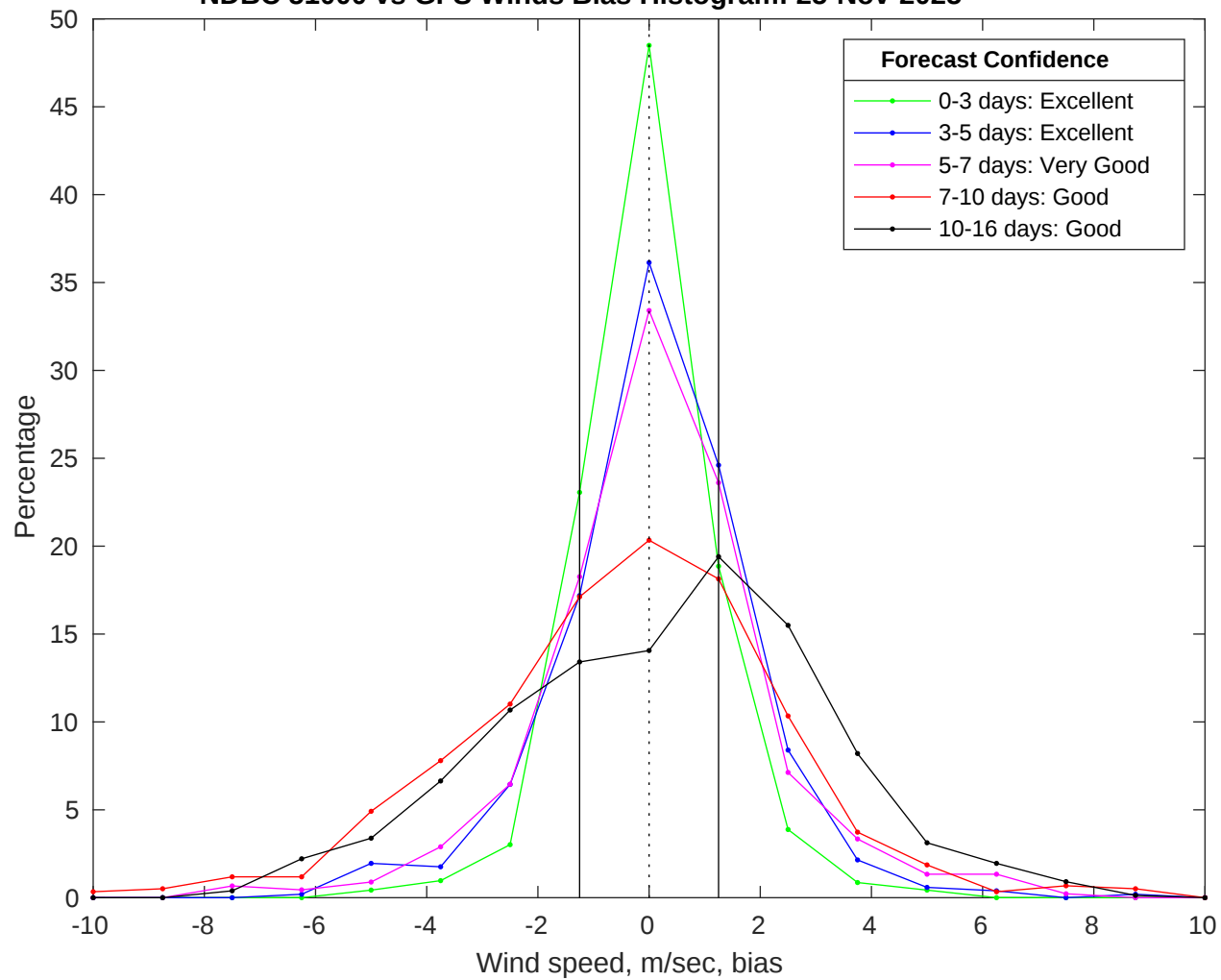
NDBC 51000 vs GFS Winds Bias Histogram: 25-Nov-2025
