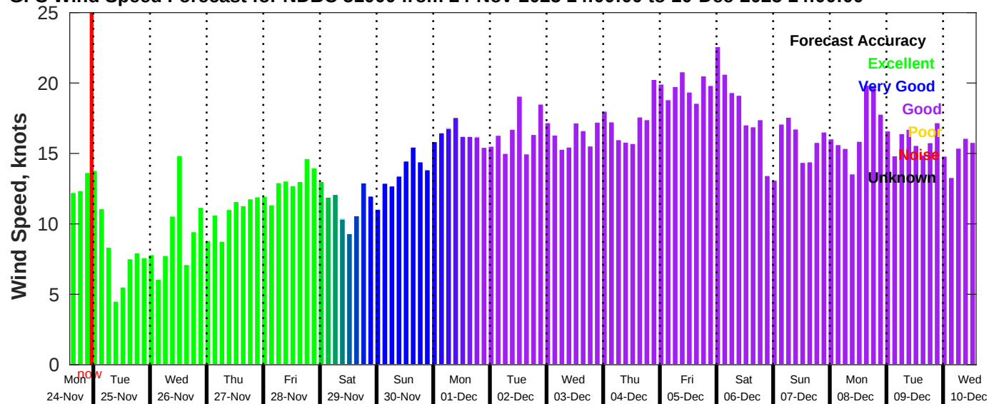
GFS Wind Speed Forecast for NDBC 51000 from 24-Nov-2025 14:00:00 to 10-Dec-2025 14:00:00
