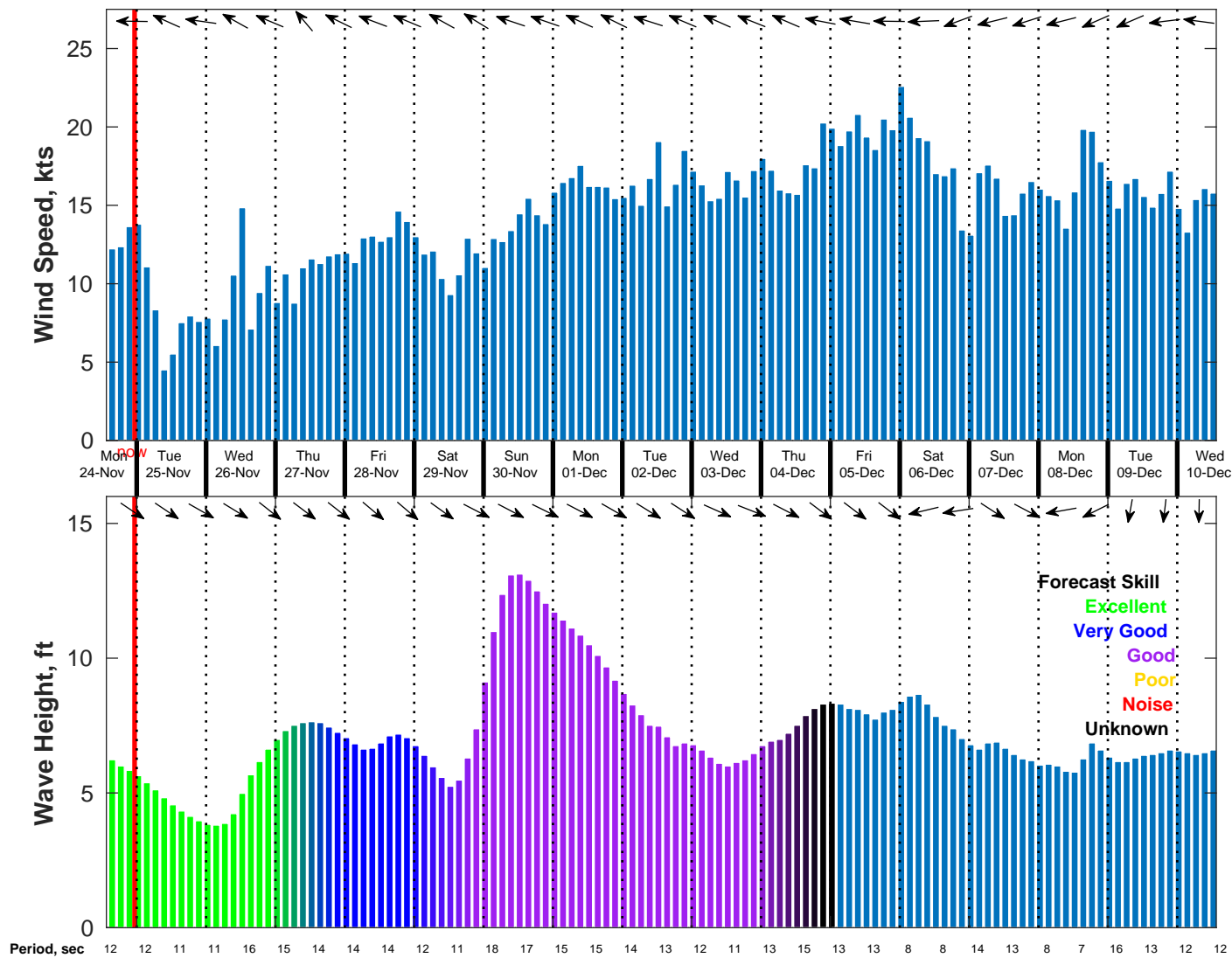
Wind & Wave Forecast for NDBC 51000 from 24-Nov-2025 14:00:00 to 10-Dec-2025 14:00:00
