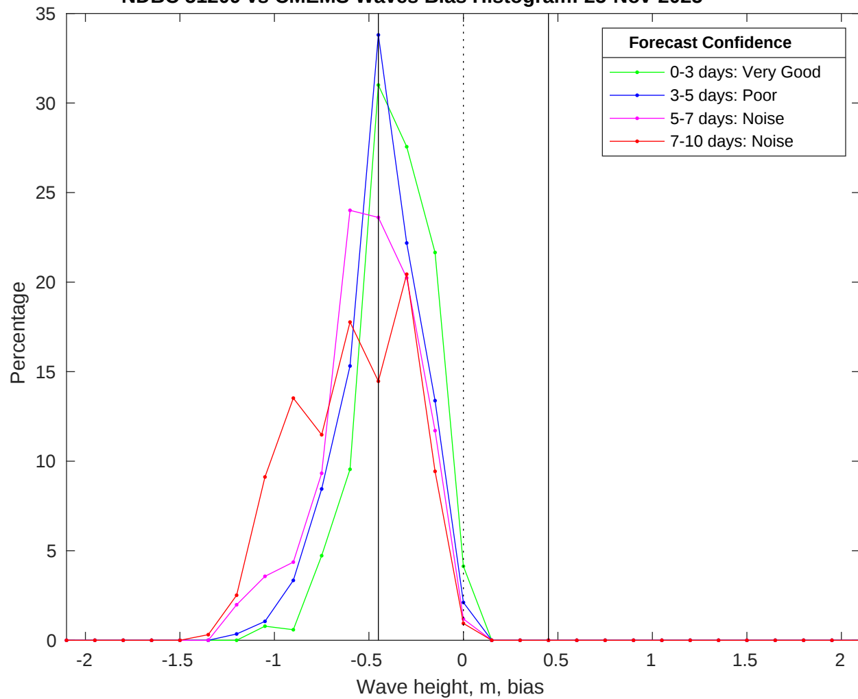
NDBC 51209 vs CMEMS Waves Bias Histogram: 25-Nov-2025
