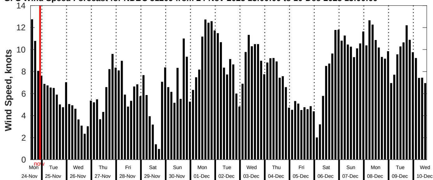
GFS Wind Speed Forecast for NDBC 51209 from 24-Nov-2025 13:00:00 to 10-Dec-2025 13:00:00
