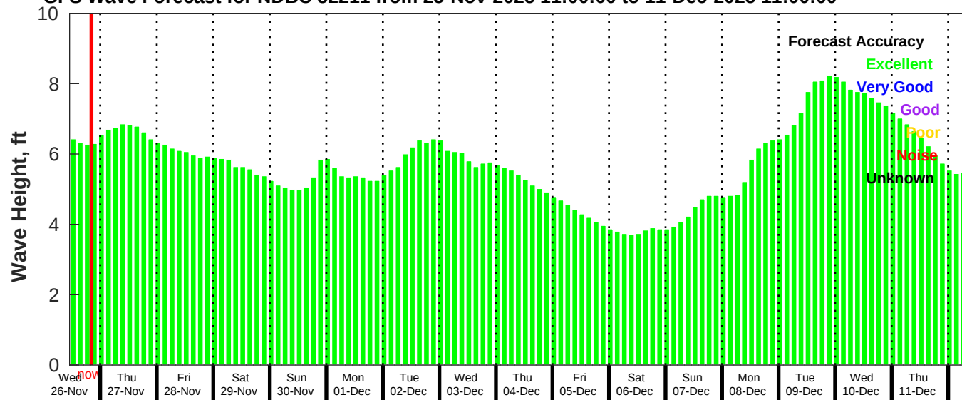
GFS Wave Forecast for NDBC 52211 from 25-Nov-2025 11:00:00 to 11-Dec-2025 11:00:00
