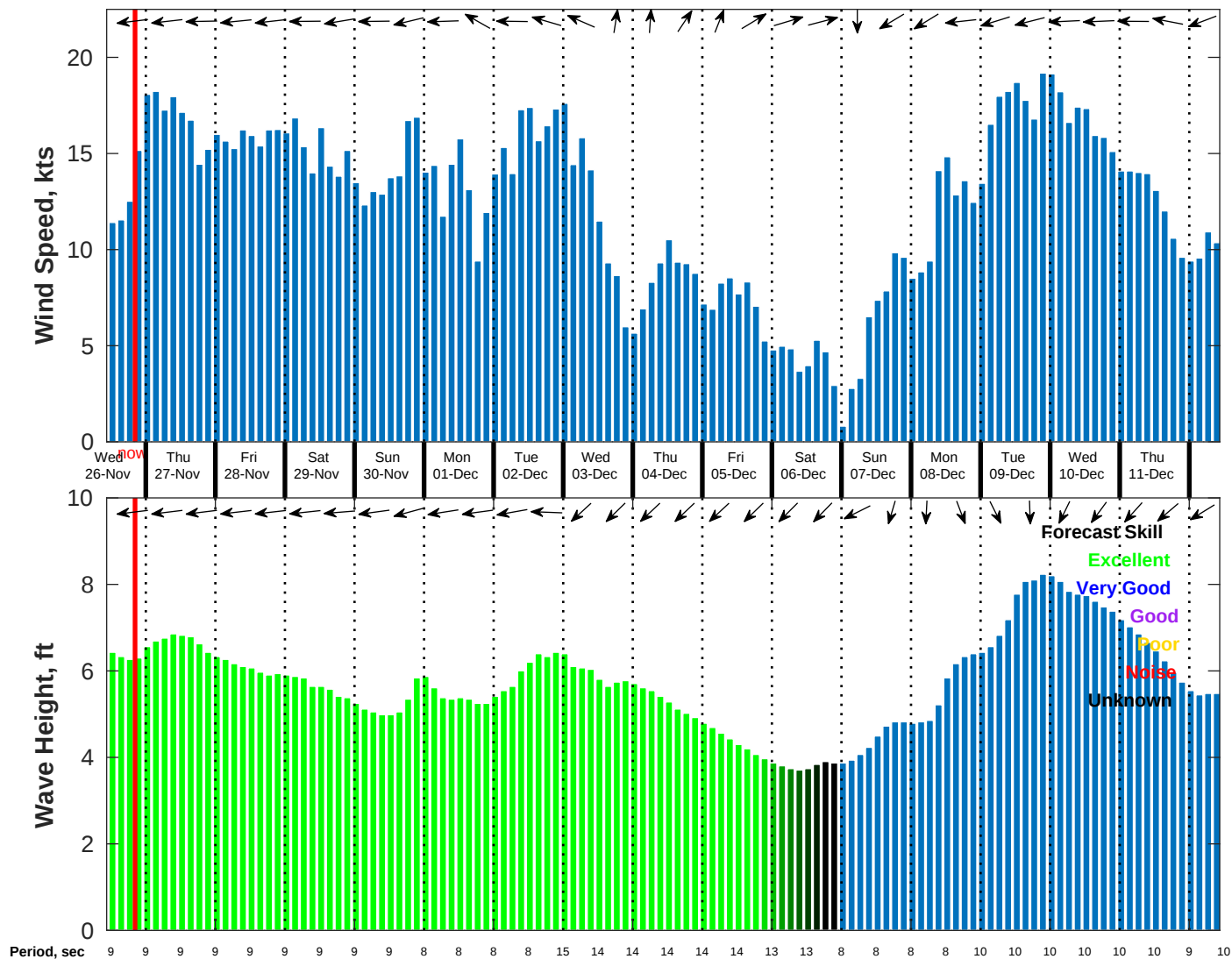
Wind & Wave Forecast for NDBC 52211 from 25-Nov-2025 11:00:00 to 11-Dec-2025 11:00:00
