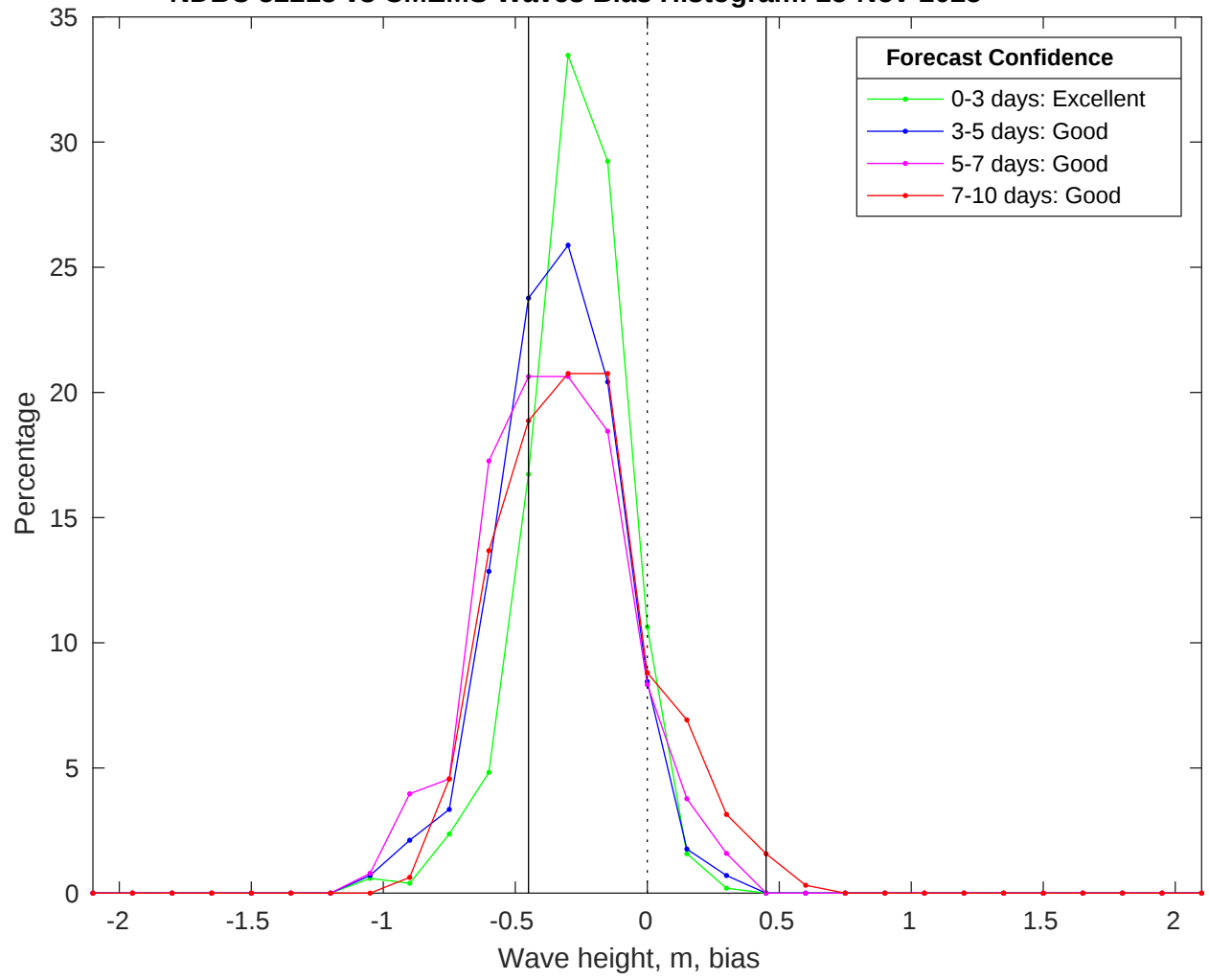
NDBC 52213 vs CMEMS Waves Bias Histogram: 25-Nov-2025
