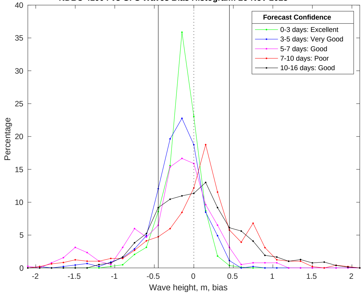
NDBC 41004 vs GFS Waves Bias Histogram: 26-Nov-2025
