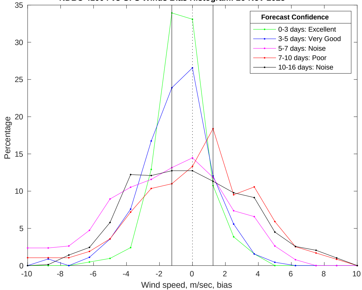
NDBC 41004 vs GFS Winds Bias Histogram: 26-Nov-2025
