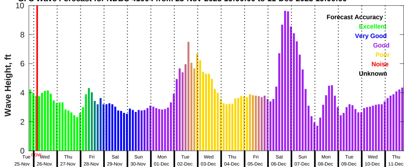
GFS Wave Forecast for NDBC 41004 from 25-Nov-2025 19:00:00 to 11-Dec-2025 19:00:00
