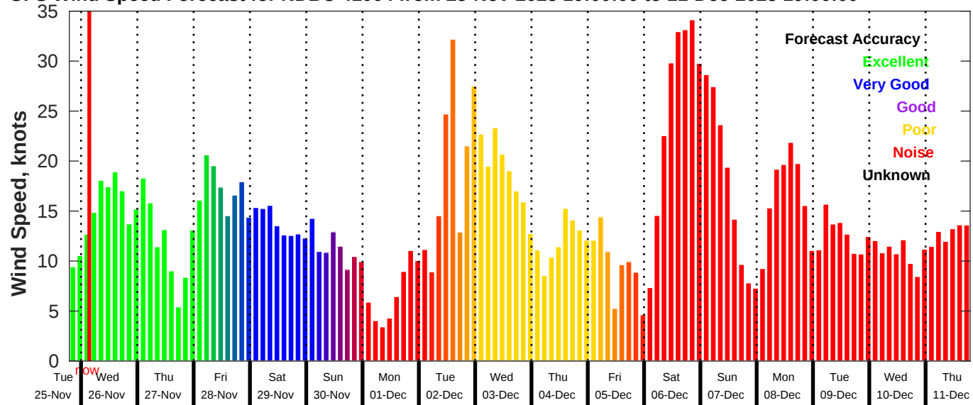
GFS Wind Speed Forecast for NDBC 41004 from 25-Nov-2025 19:00:00 to 11-Dec-2025 19:00:00
