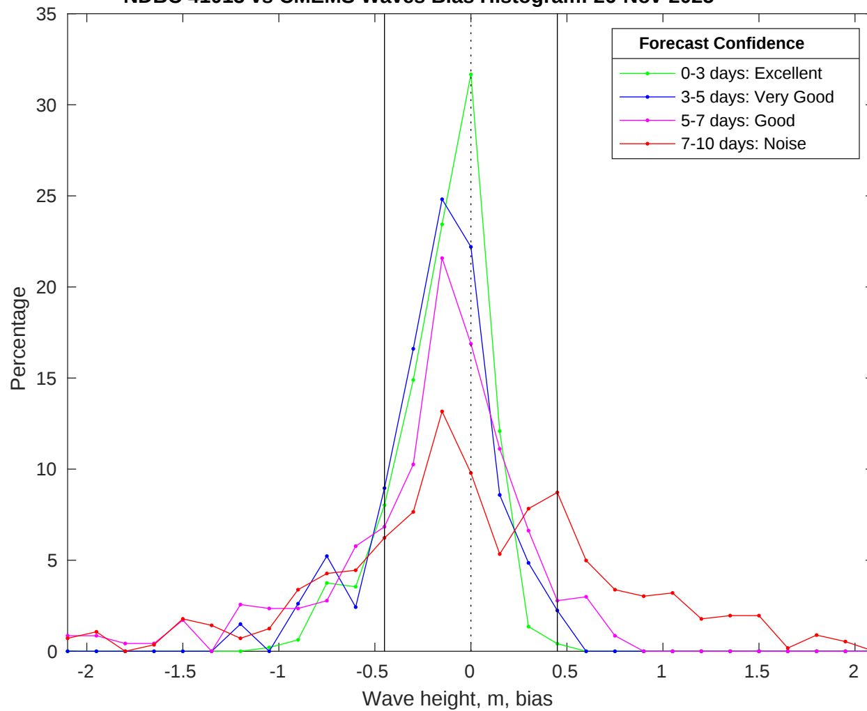
NDBC 41013 vs CMEMS Waves Bias Histogram: 26-Nov-2025
