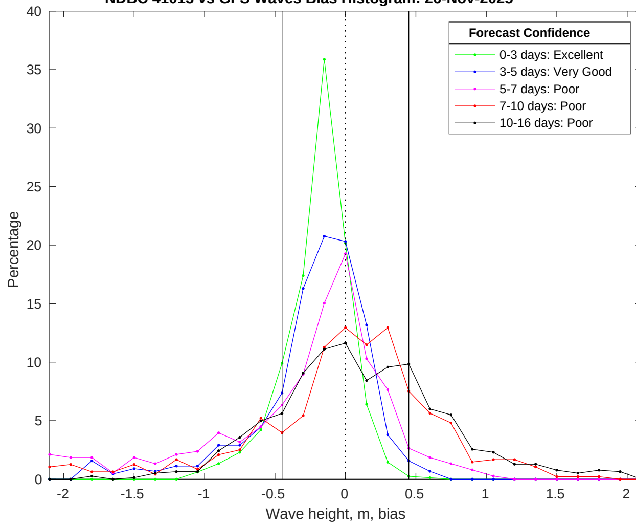
NDBC 41013 vs GFS Waves Bias Histogram: 26-Nov-2025
