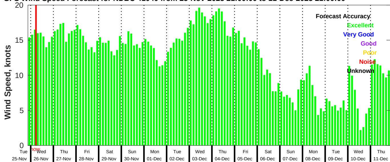
GFS Wind Speed Forecast for NDBC 41040 from 25-Nov-2025 21:00:00 to 11-Dec-2025 21:00:00
