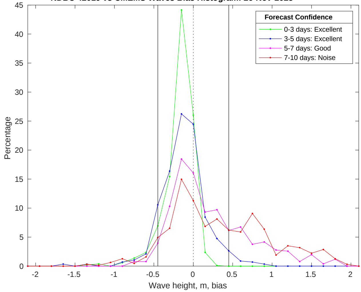
NDBC 42019 vs CMEMS Waves Bias Histogram: 26-Nov-2025
