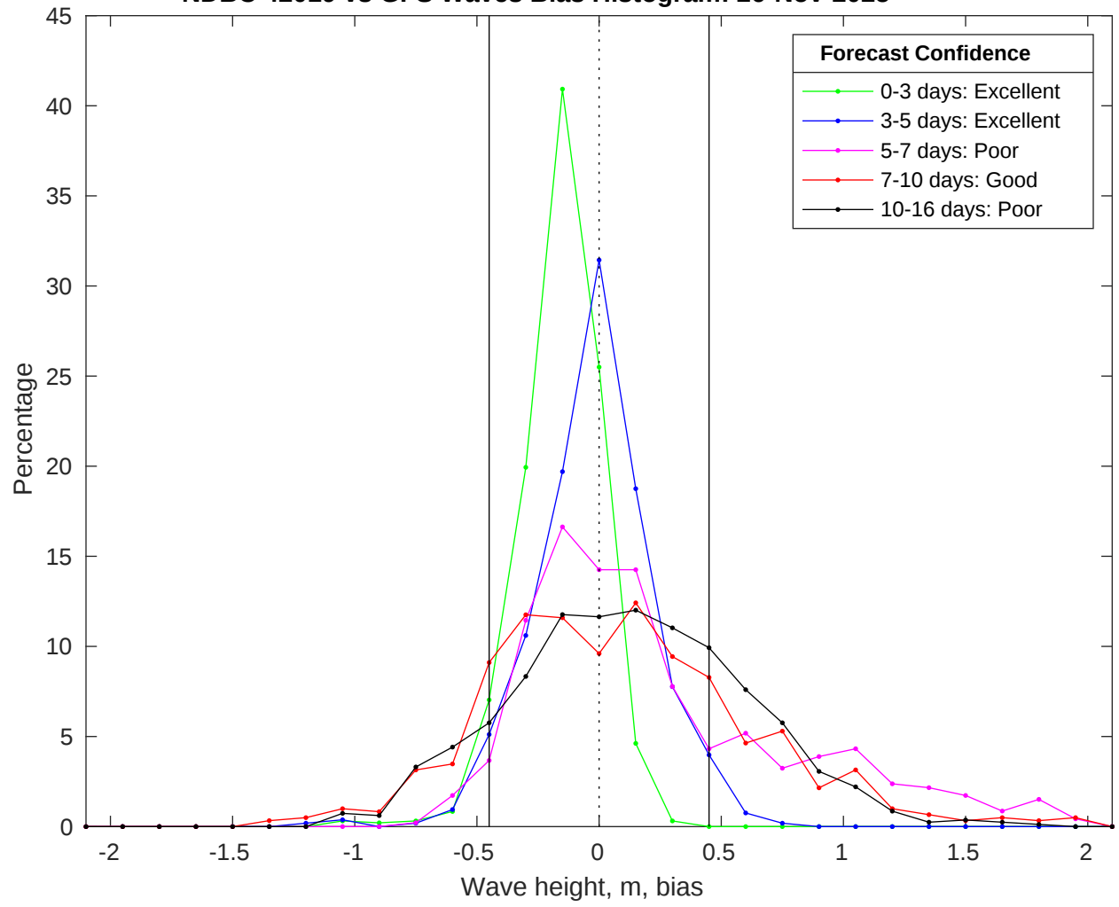
NDBC 42019 vs GFS Waves Bias Histogram: 26-Nov-2025
