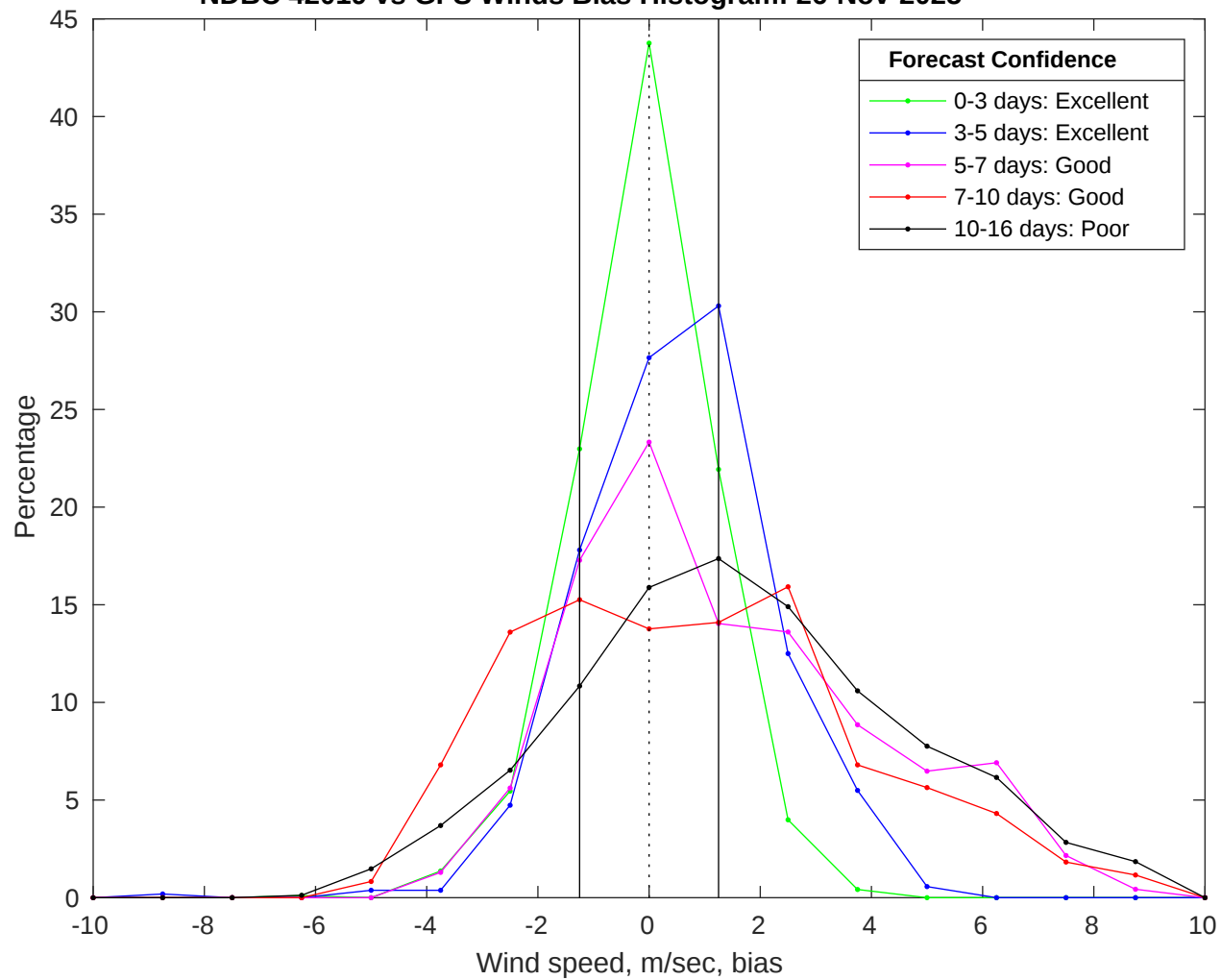
NDBC 42019 vs GFS Winds Bias Histogram: 26-Nov-2025
