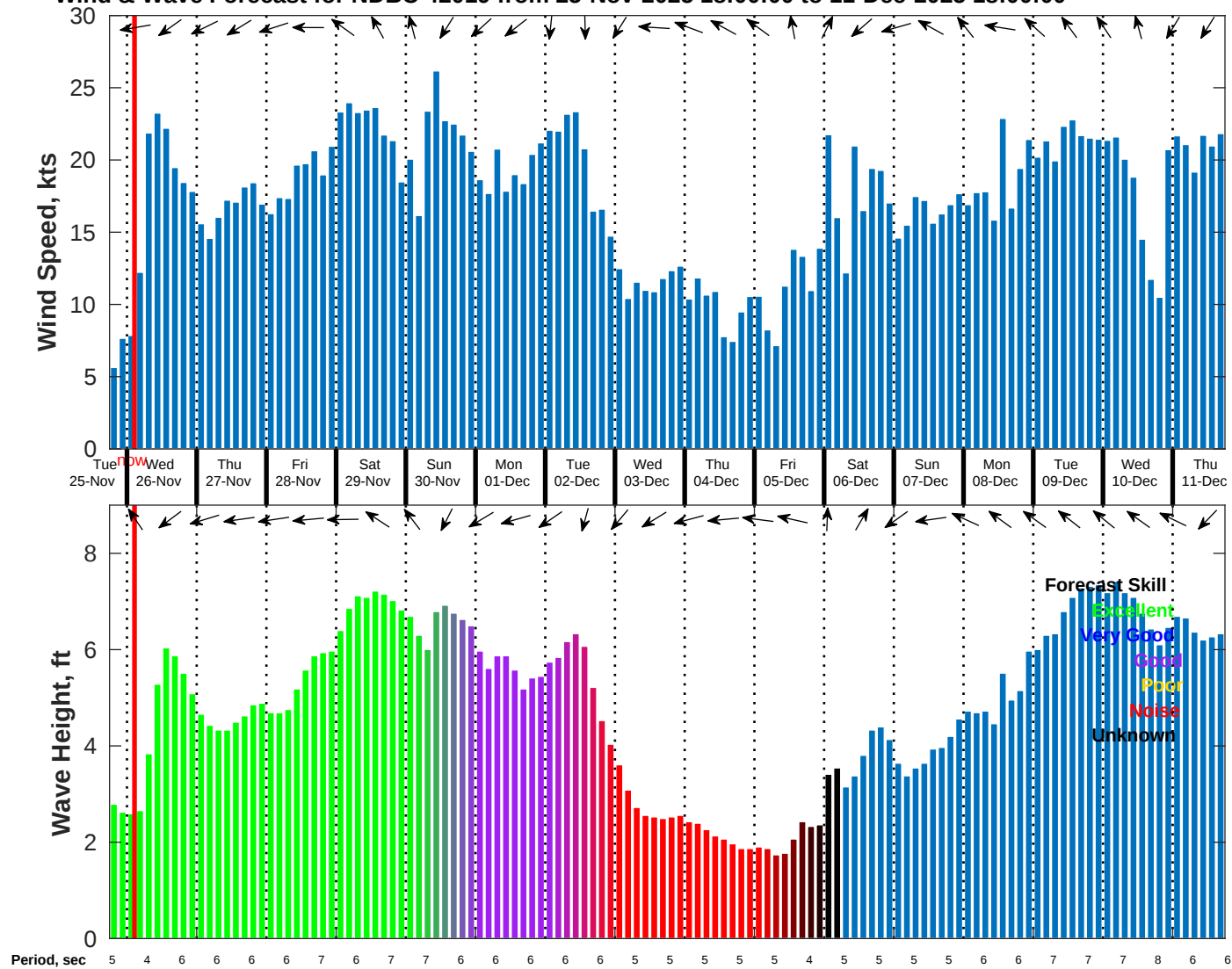
Wind & Wave Forecast for NDBC 42019 from 25-Nov-2025 18:00:00 to 11-Dec-2025 18:00:00
