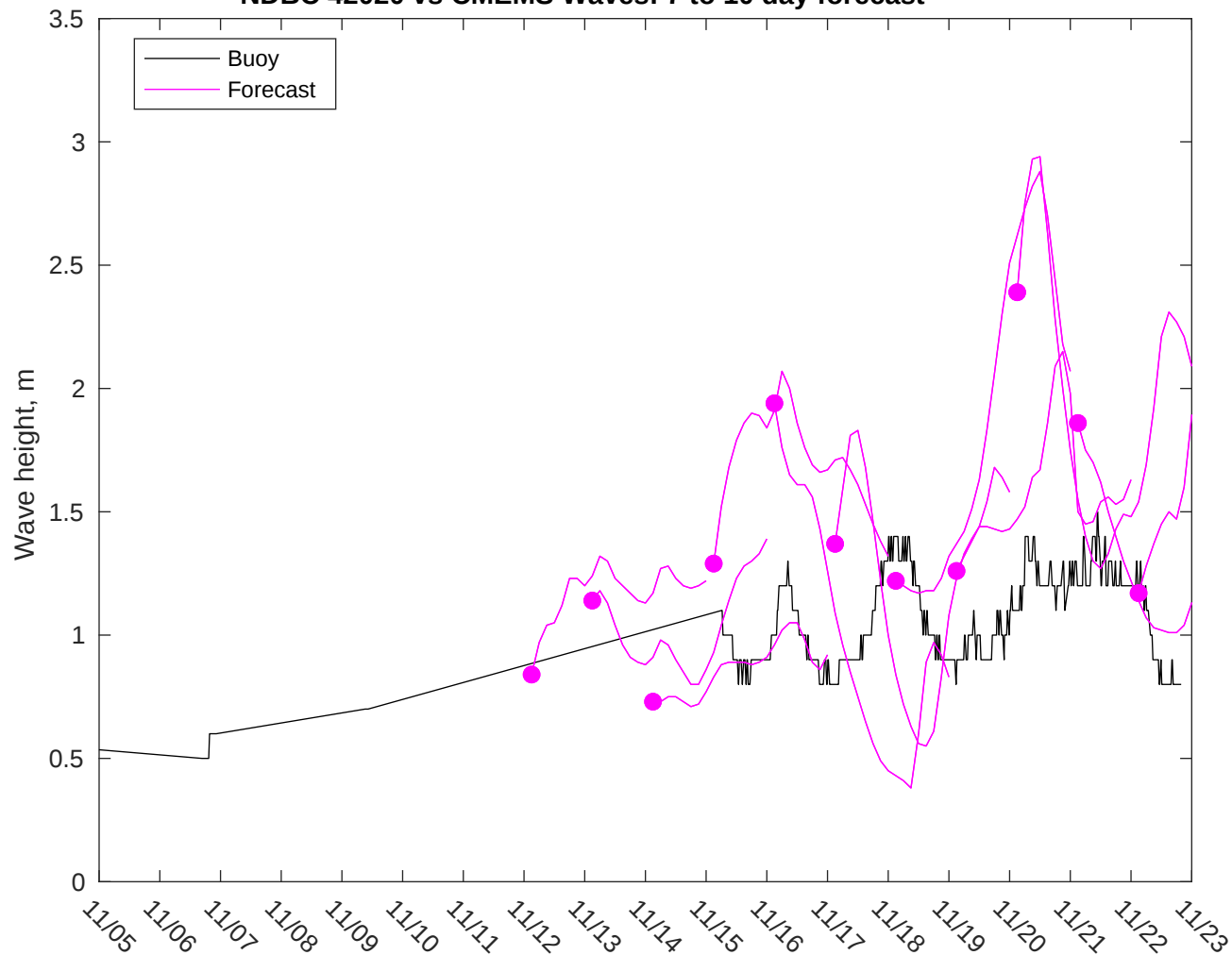
NDBC 42020 vs CMEMS Waves: 7 to 10 day forecast
