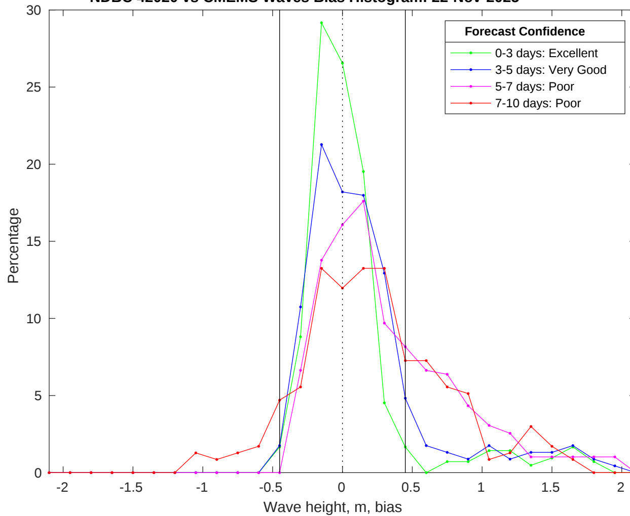
NDBC 42020 vs CMEMS Waves Bias Histogram: 22-Nov-2025
