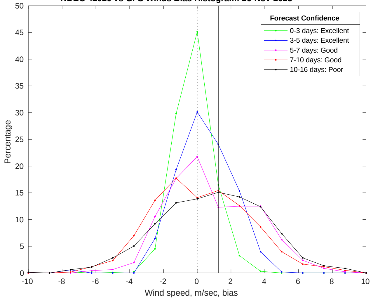
NDBC 42020 vs GFS Winds Bias Histogram: 26-Nov-2025
