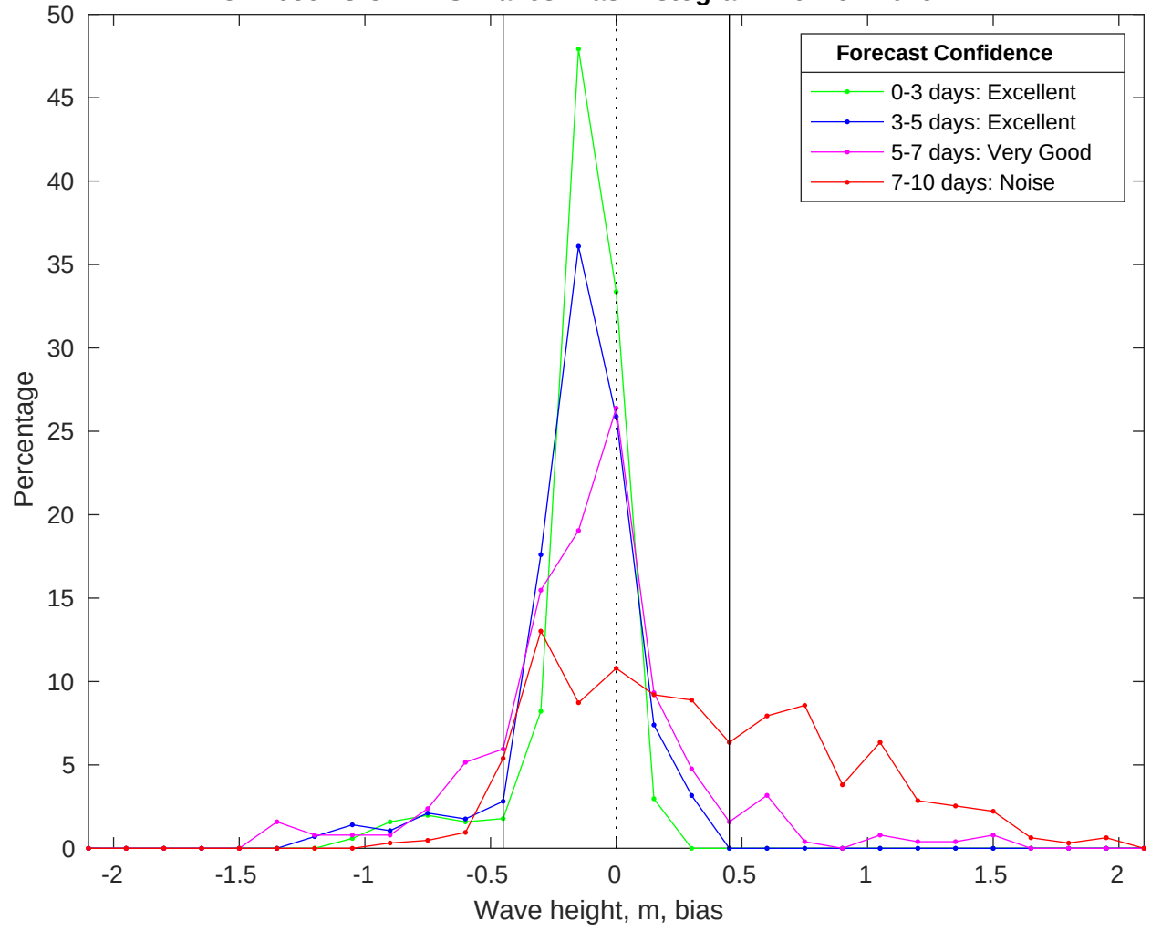
NDBC 42036 vs CMEMS Waves Bias Histogram: 26-Nov-2025
