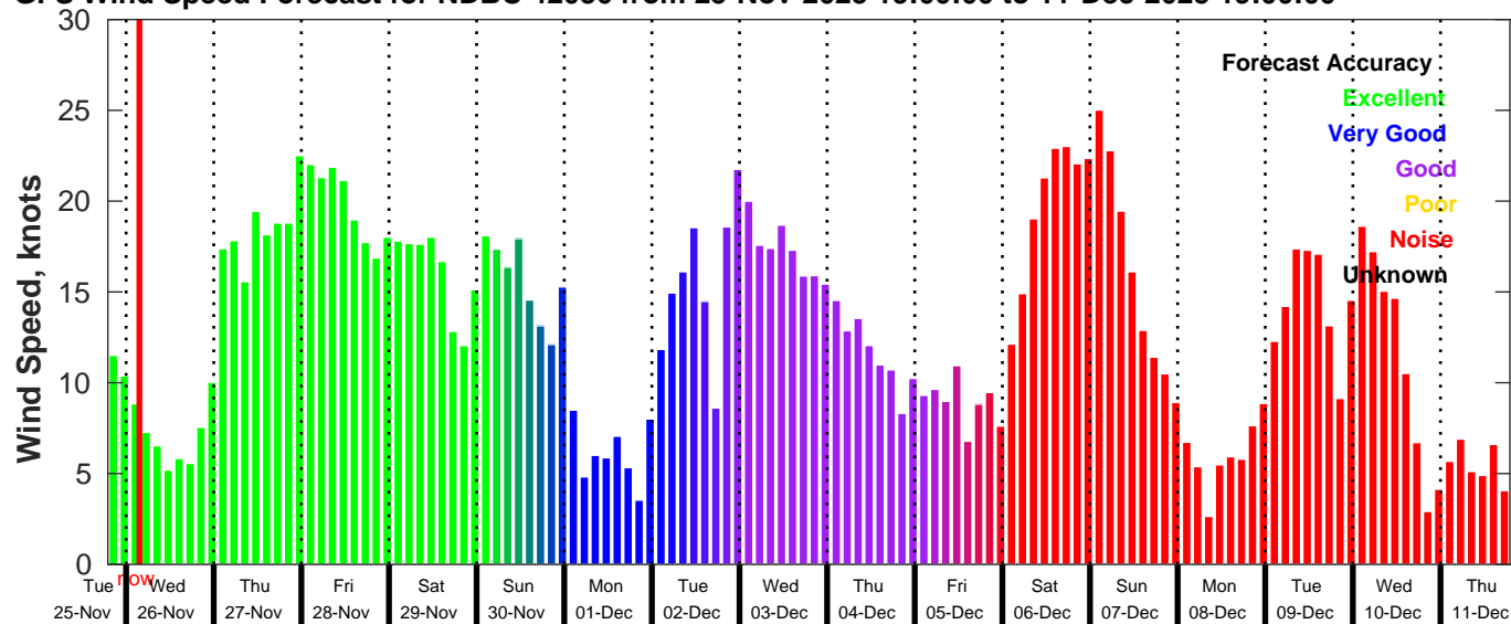
GFS Wind Speed Forecast for NDBC 42036 from 25-Nov-2025 19:00:00 to 11-Dec-2025 19:00:00
