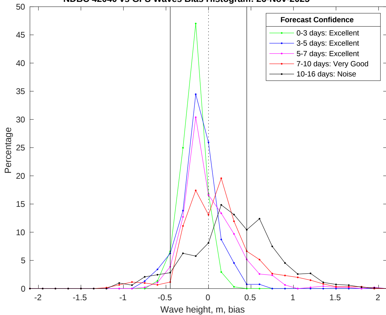
NDBC 42040 vs GFS Waves Bias Histogram: 26-Nov-2025
