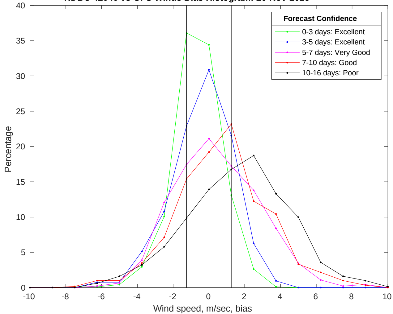
NDBC 42040 vs GFS Winds Bias Histogram: 26-Nov-2025
